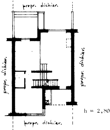
PIANO TERRA
