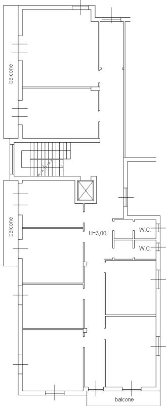
PIANO QUARTO
