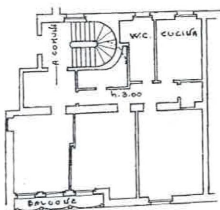
PIANO QUARTO
