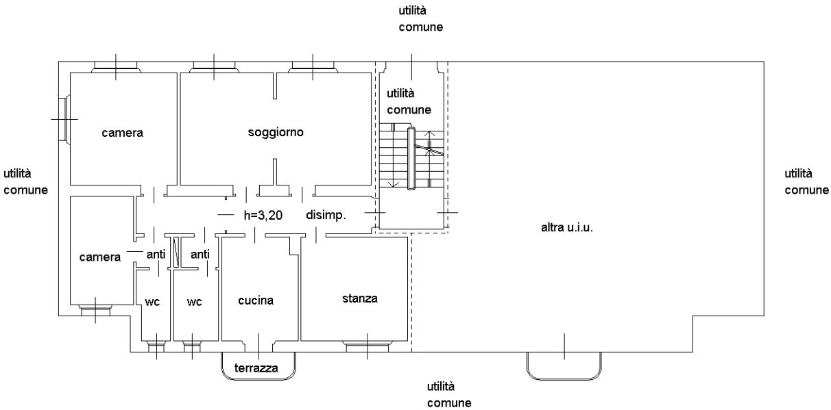
Piano rialzato h 3.20m
